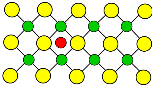
interstitial impurity
