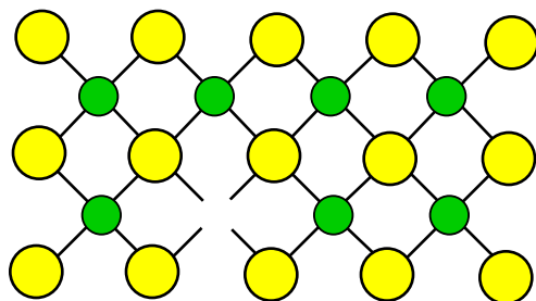
cation vacancy
