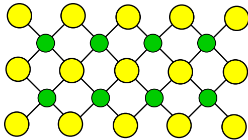
perfect lattice
