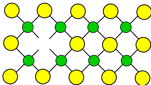
anion vacancy
